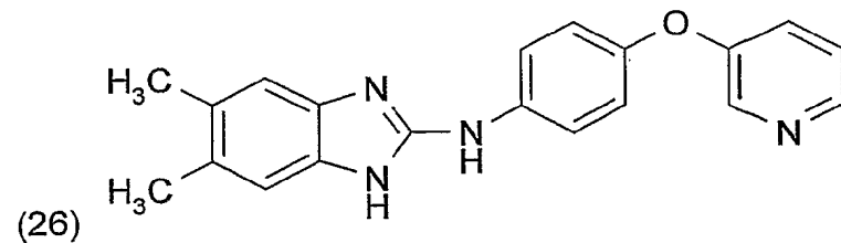
(5,6-Dimethyl-1H-benzimidazol-2-yl)-[4-(pyridin-3-yloxy)-phenyl]-amin
